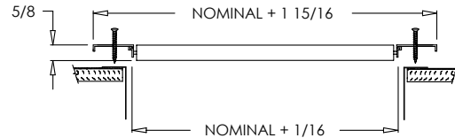
935 Rectangle (Stamped Steel One Piece Frame)
