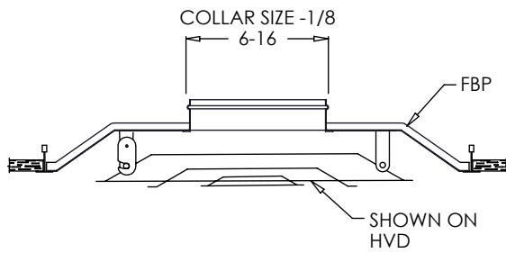
FBP Typical Installation
