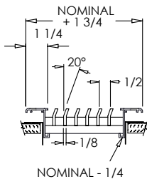
LS 1/2 20° X FRAME
