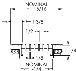
LS 1/2 0° STANDARD FRAME
